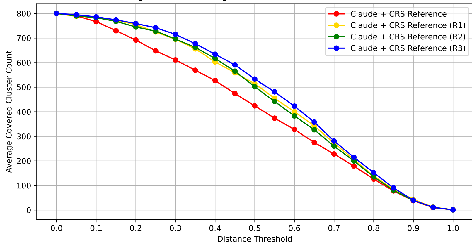
Average Cluster Coverage vs Distance Threshold (Seeds 1-1)
